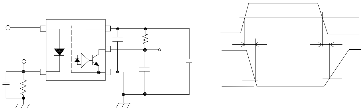
Fig.9: Switching Time Test Circuit and Waveform
