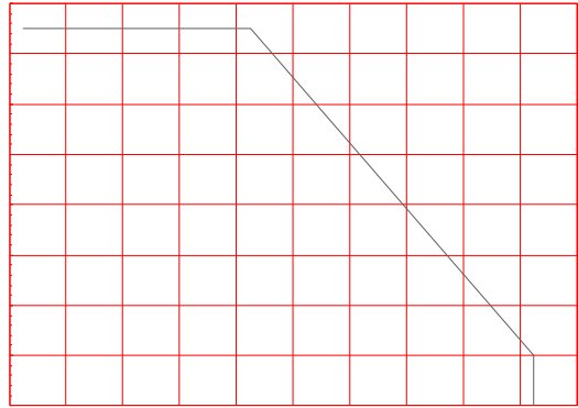
Collector Power Dissipation vs. Ambient Temperature
