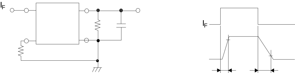
FIG.7: Response Time Test Circuit, Waveform
