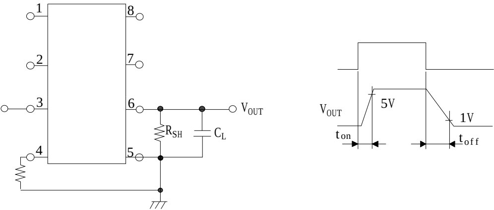
FIG.7: Response Time Test Circuit, Waveform
